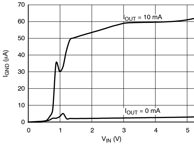
Figure 11. Supply Current vs. Input Voltage, 1.2 V Version
