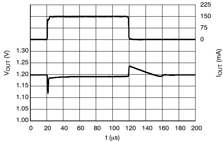
Figure 32. Load Transients, 2.8 V Version, I_{OUT} = 1 - 50 \text{ mA} , t_R = t_F = 0.5 \mu\text{s} , V_{IN} = 3.8 \text{ V} , AE = V_{IN} \text{ V}
